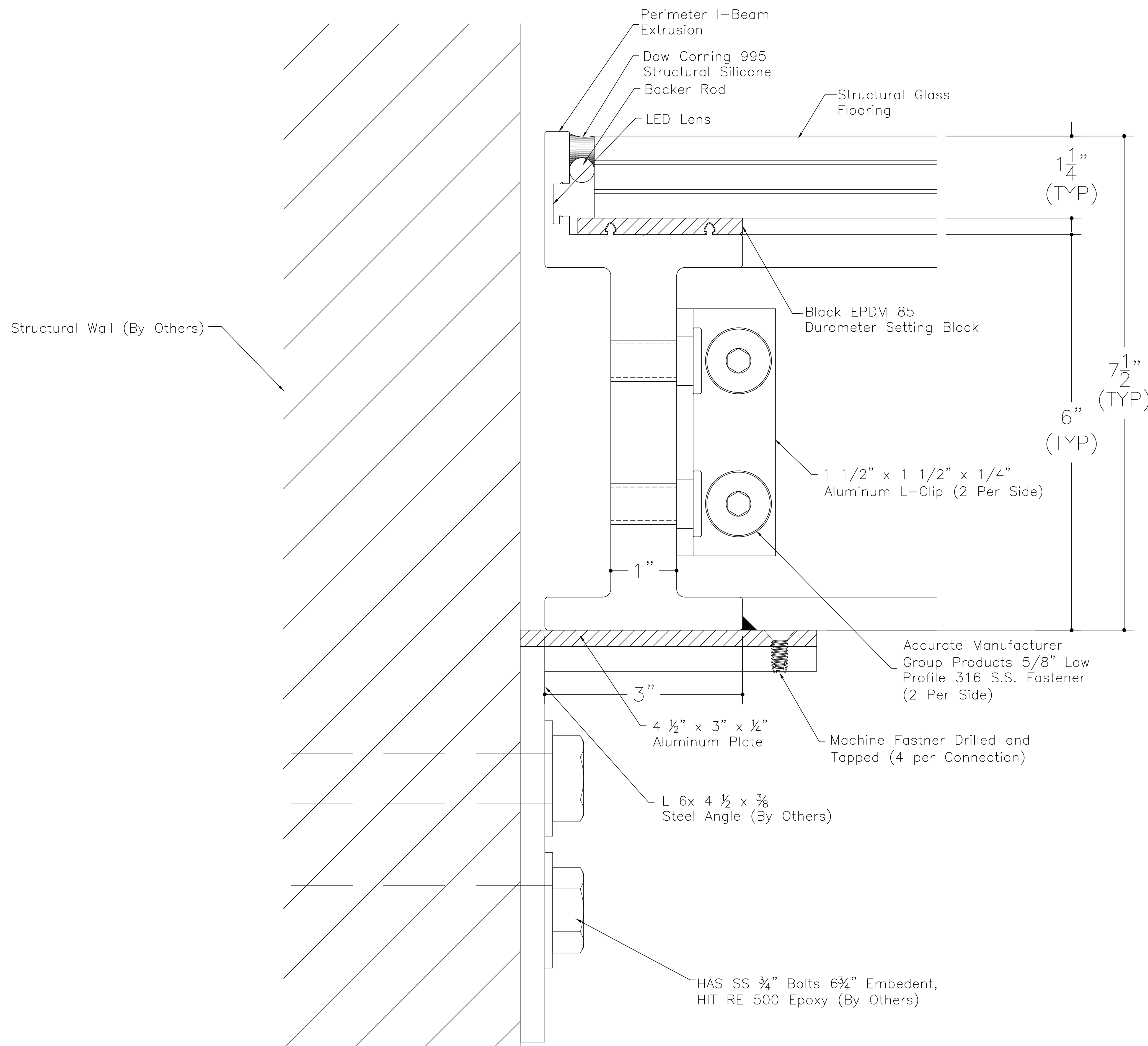
SkyFloor® Deck System Typical Wall Connection
