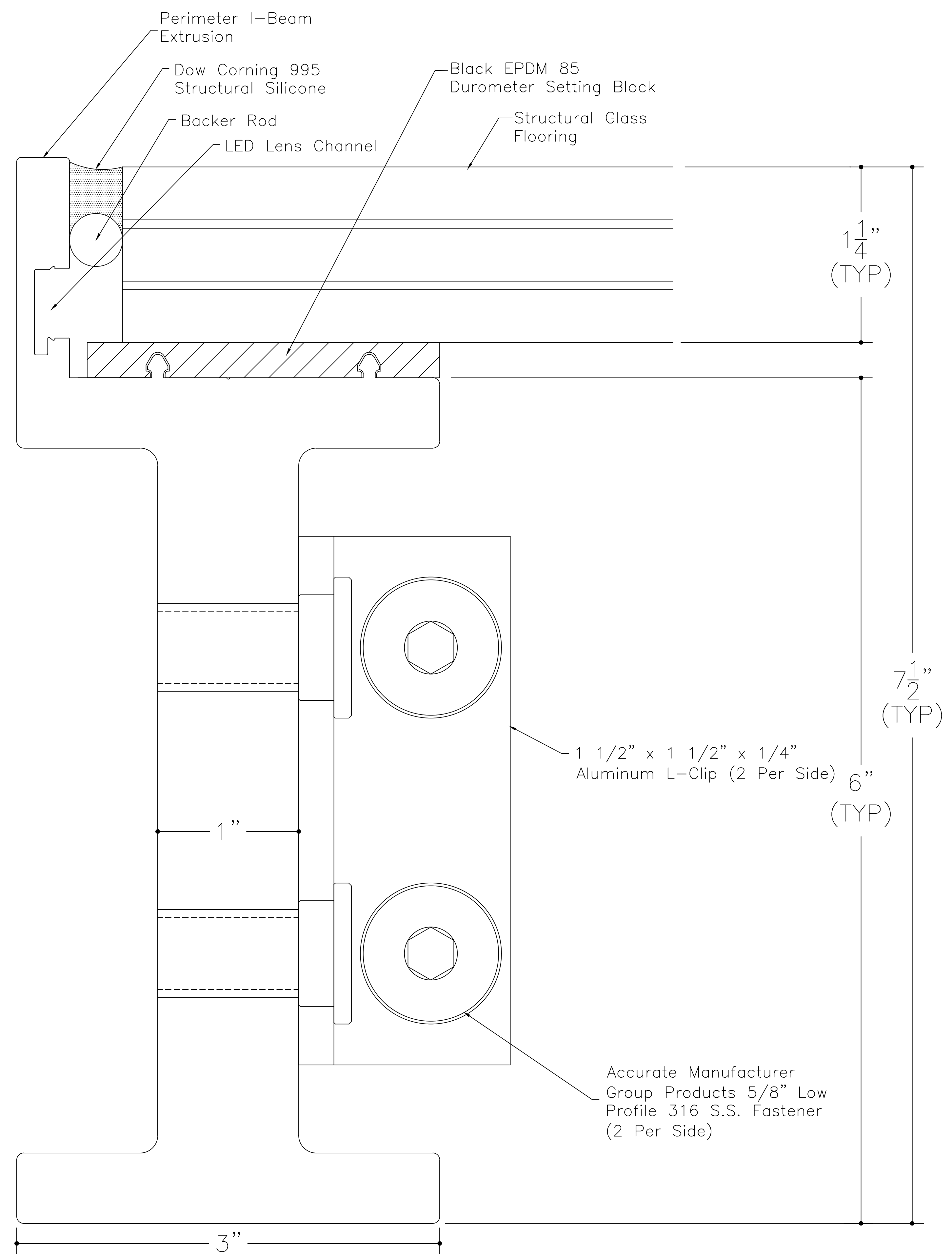
SkyFloor® Deck System Perimeter Detail
