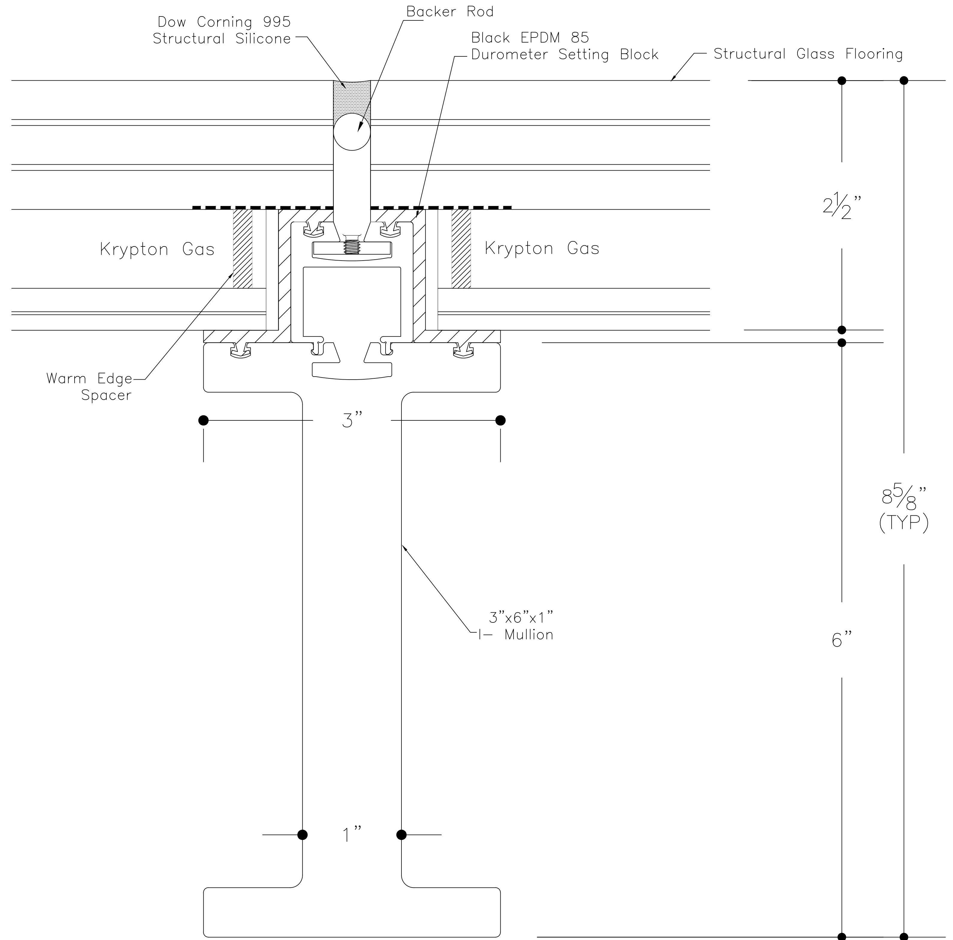
① SkyFloor® Series 2000 I Mullion with Single Spacer
