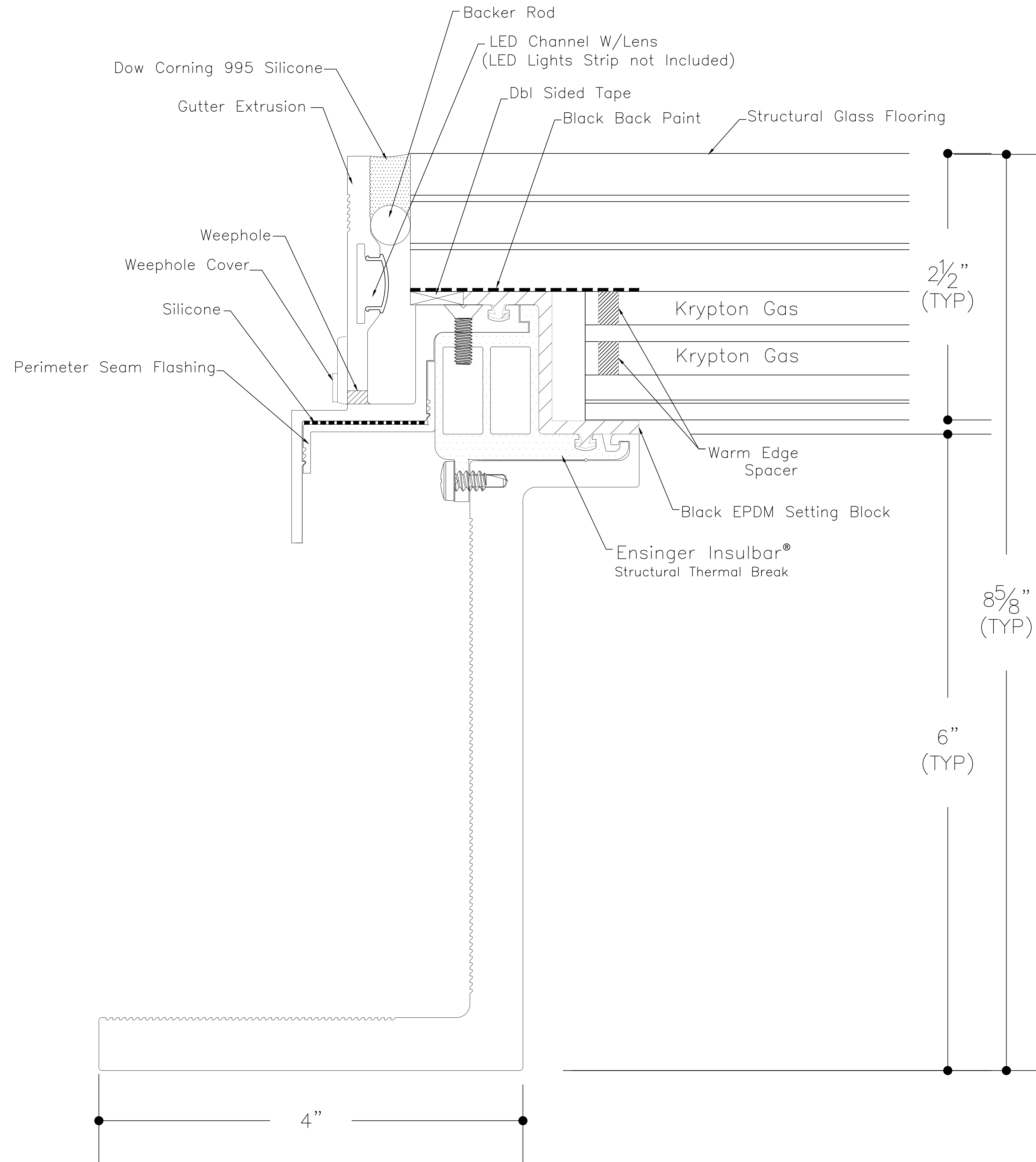
① SkyFloor® Series 2000 Pedestal perimeter with Double Spacer
