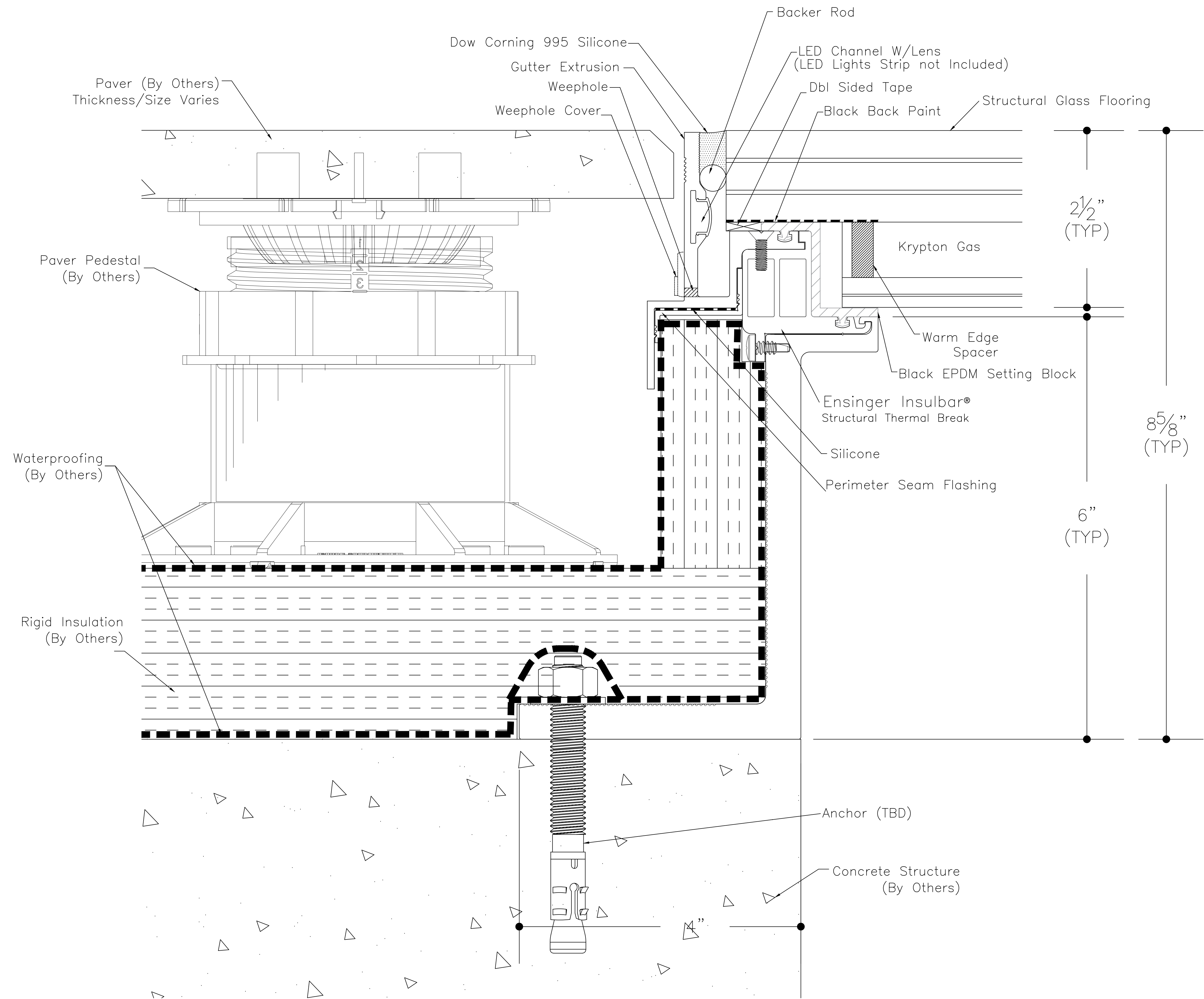
① SkyFloor® Series 2000 Pedestal perimeter with Single Spacer
