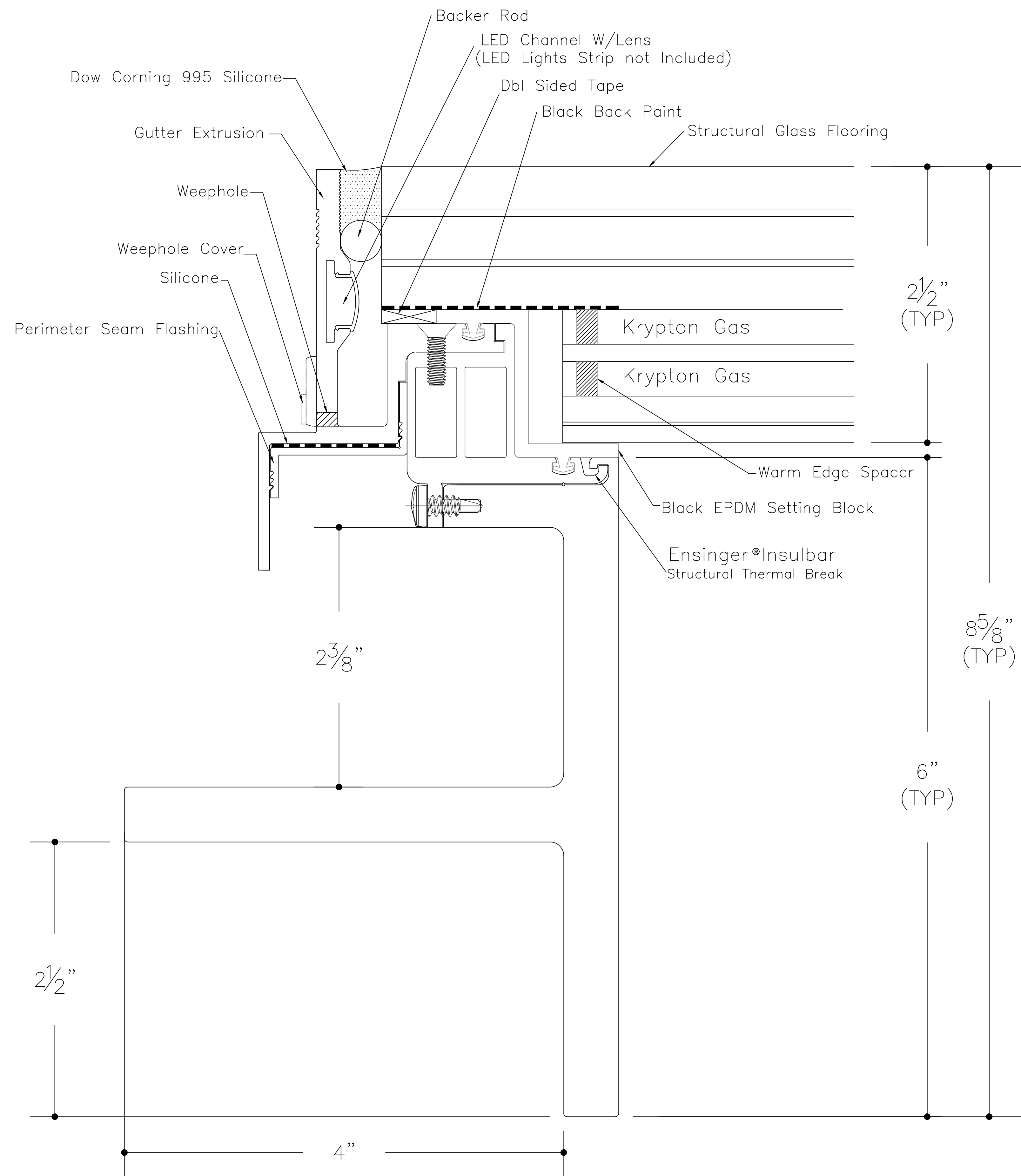
① SkyFloor® Series 2000 Recessed perimeter with Double Spacer
