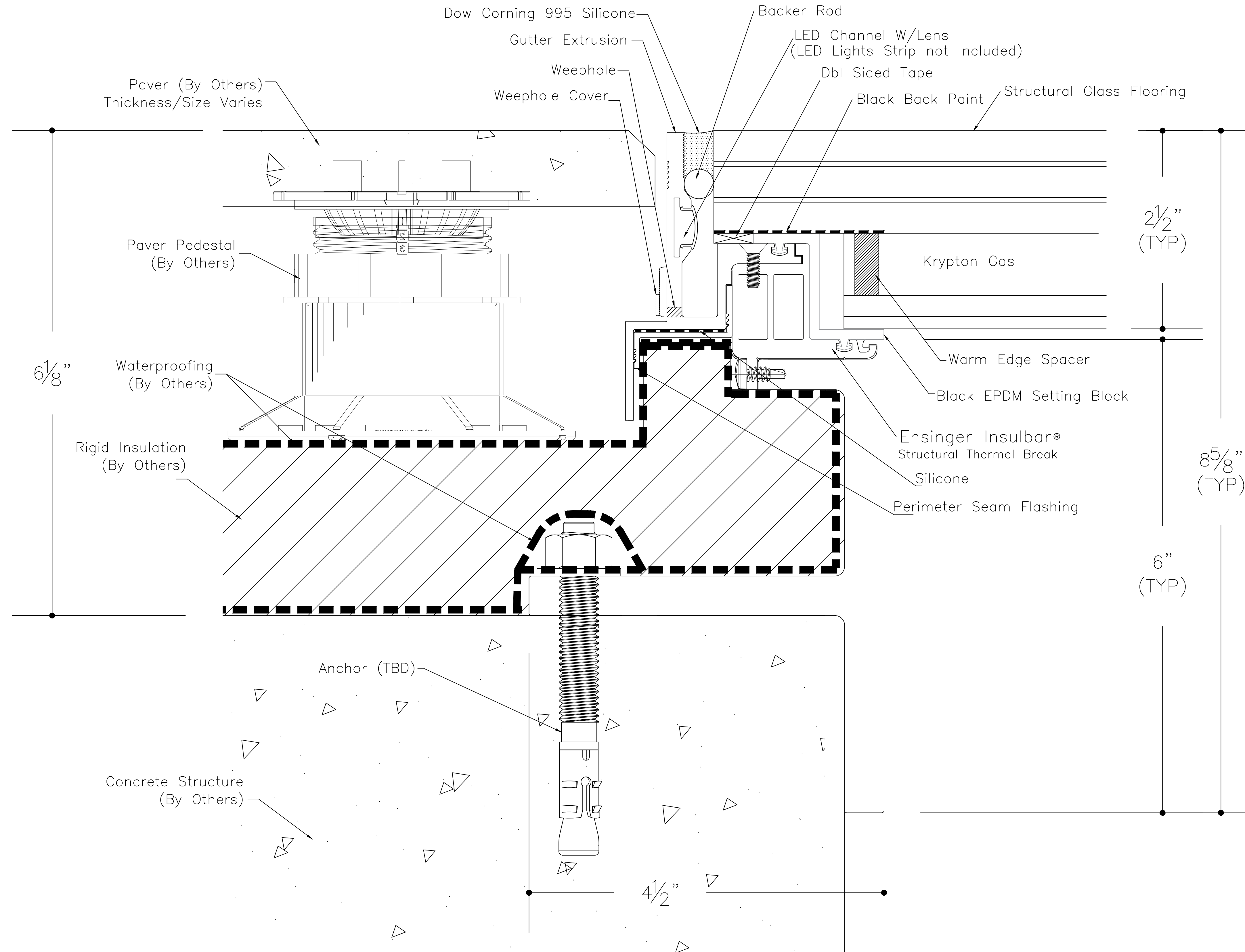
① SkyFloor® Series 2000 Recessed perimeter with Single Spacer
