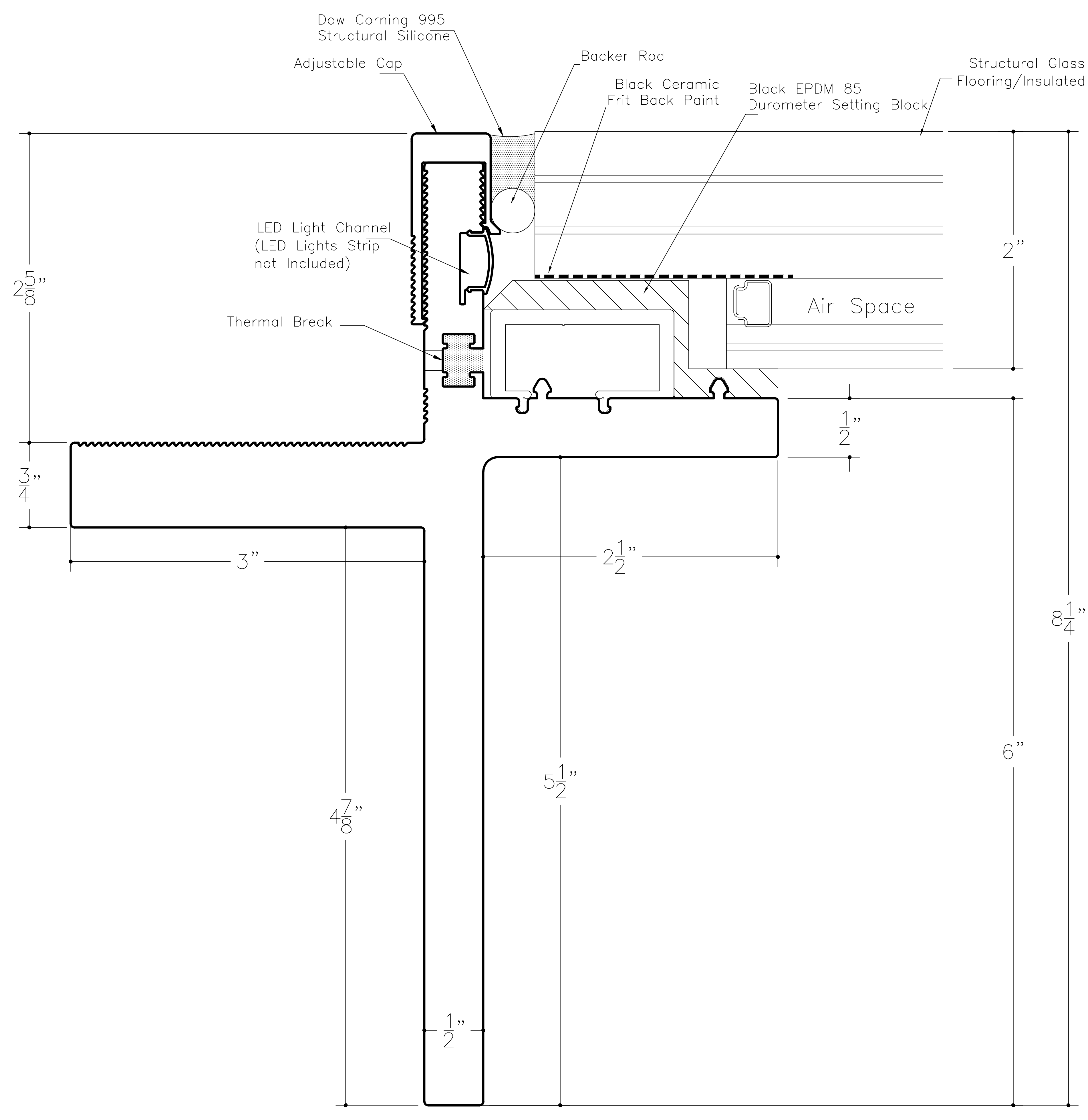
SkyFloor® Recessed Perimeter
